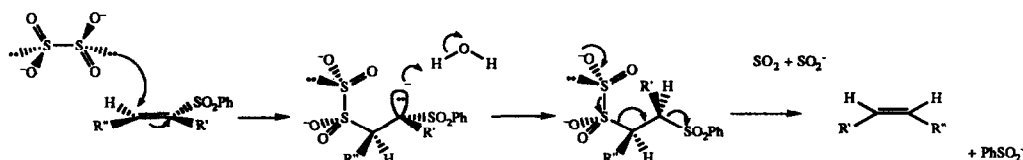
Scheme 5 - Mechanism for Desulfonylation of Vinyl Sulfones with Sodium Dithionite
